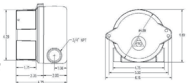
General Dimensions Side and Back Views (All Dimensions in Inche
