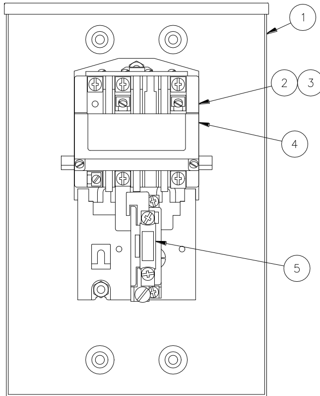
Figure 5-8. Model RC2W Parts Index
