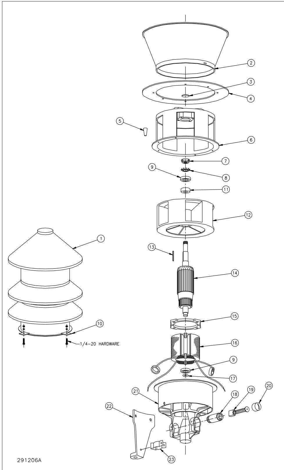
Figure 5-6. Model 2 Parts Index
